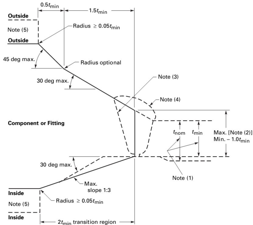
Fig. 1 Maximum Envelope for Welding End Transitions
